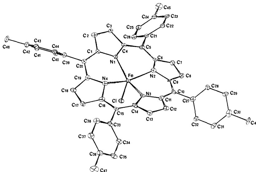
Figure 1. Perspective view and atom numbering scheme of the \text{FeCl}(\text{TTP})^+ cation. Thermal ellipsoids are contoured at the 50% probability level ( -140^\circ\text{C} ).
